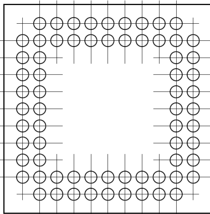
68 PGA
