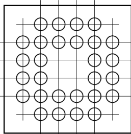
28 PGA
