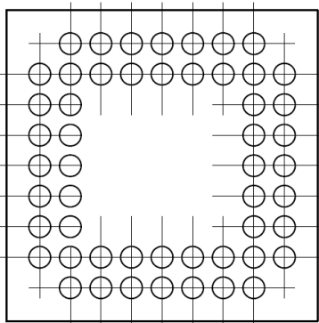
52 PGA
