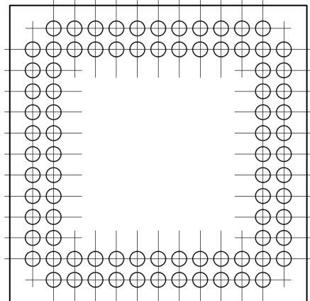
84 PGA
